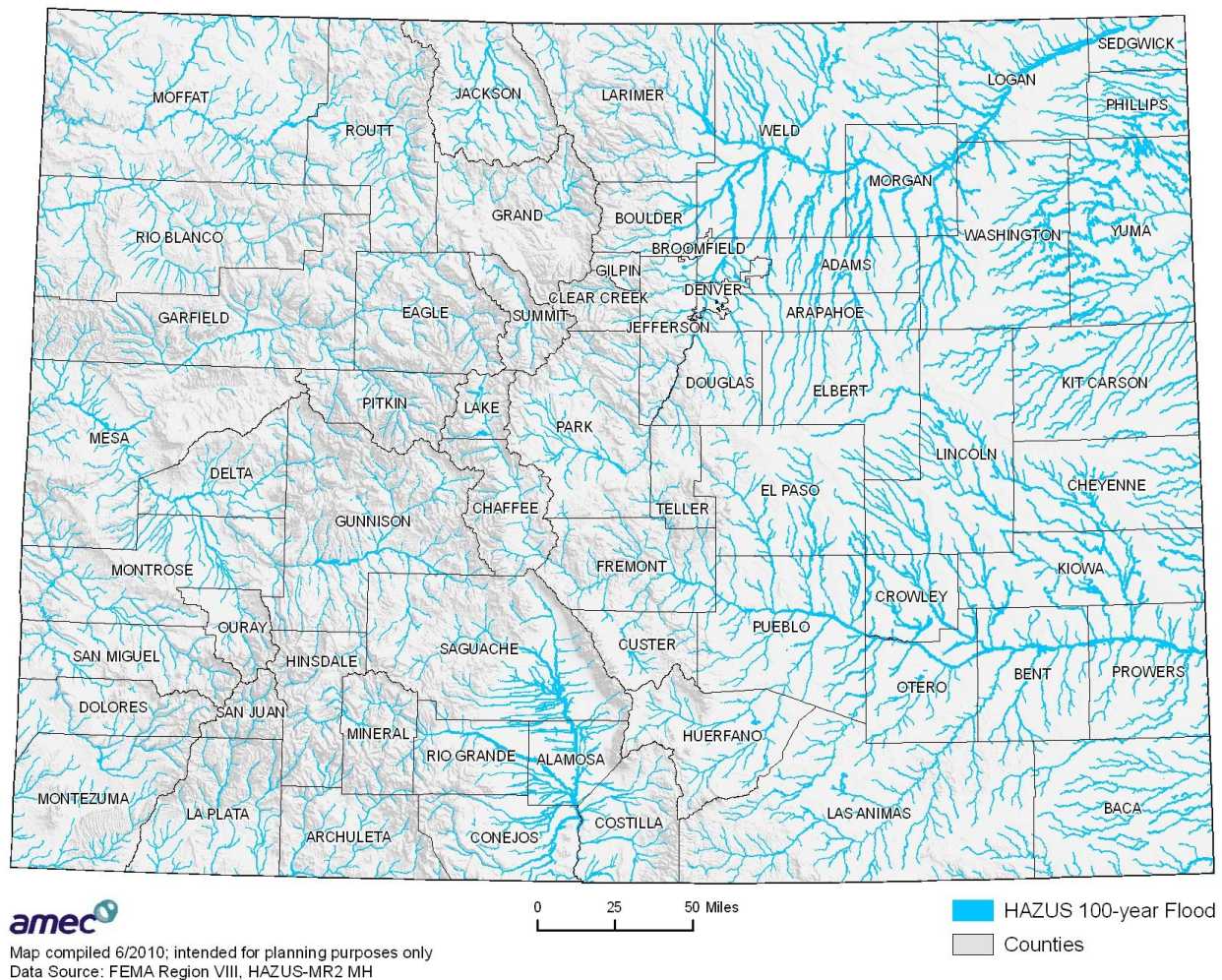
Figure 4 HAZUS-MH 100-year Floodplains in Colorado
