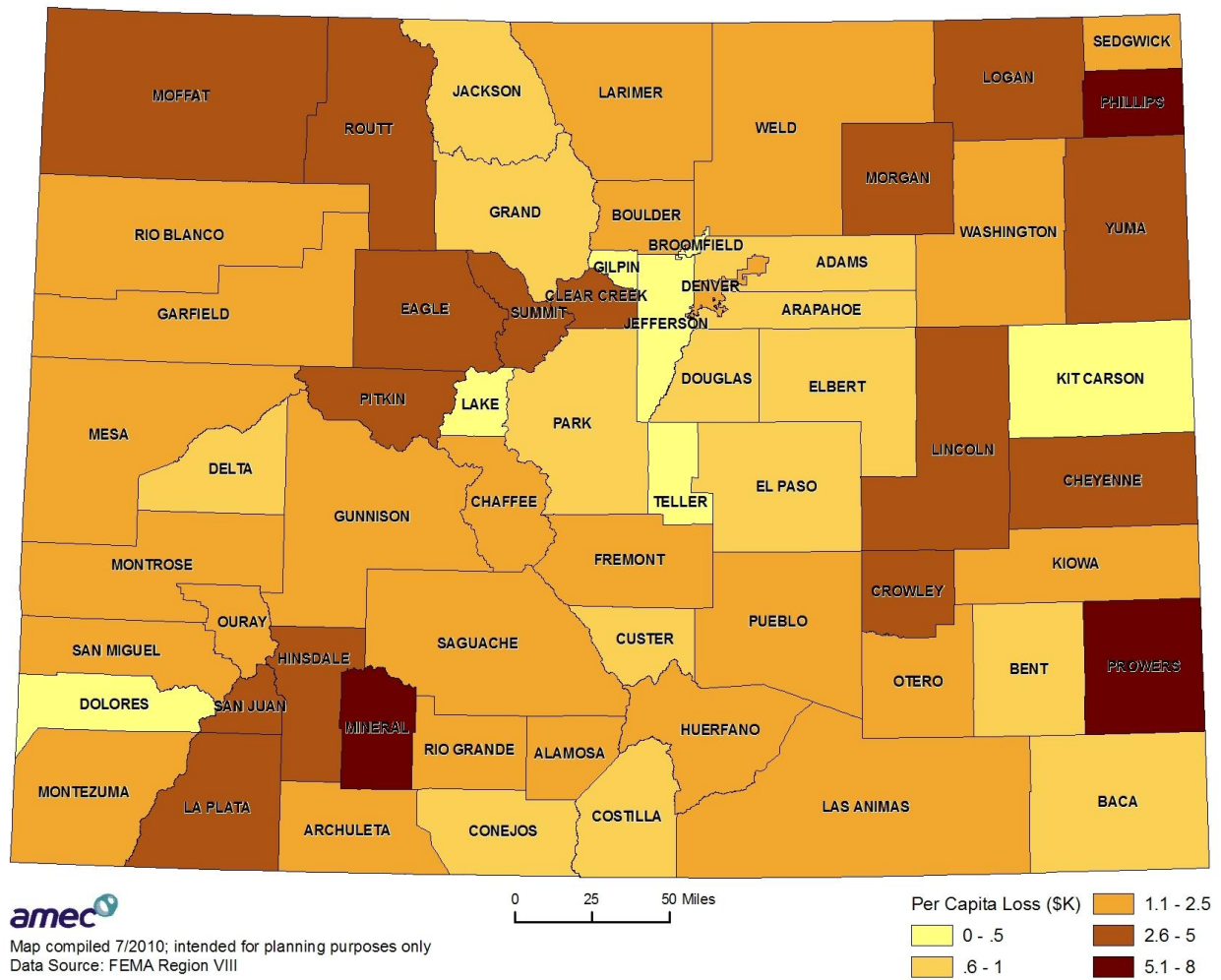
Figure 11 Per Capita Loss by County based on HAZUS
