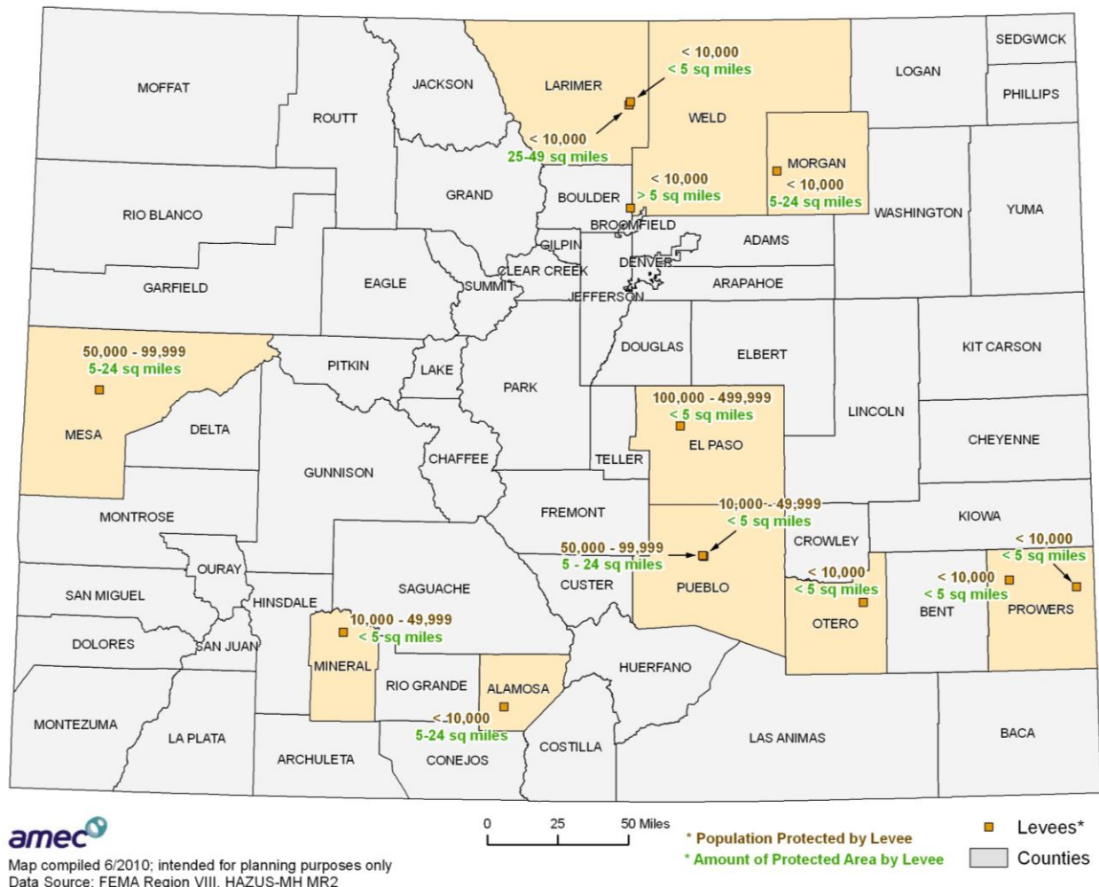
Figure 5 Colorado Levees: Protected Population and Area
