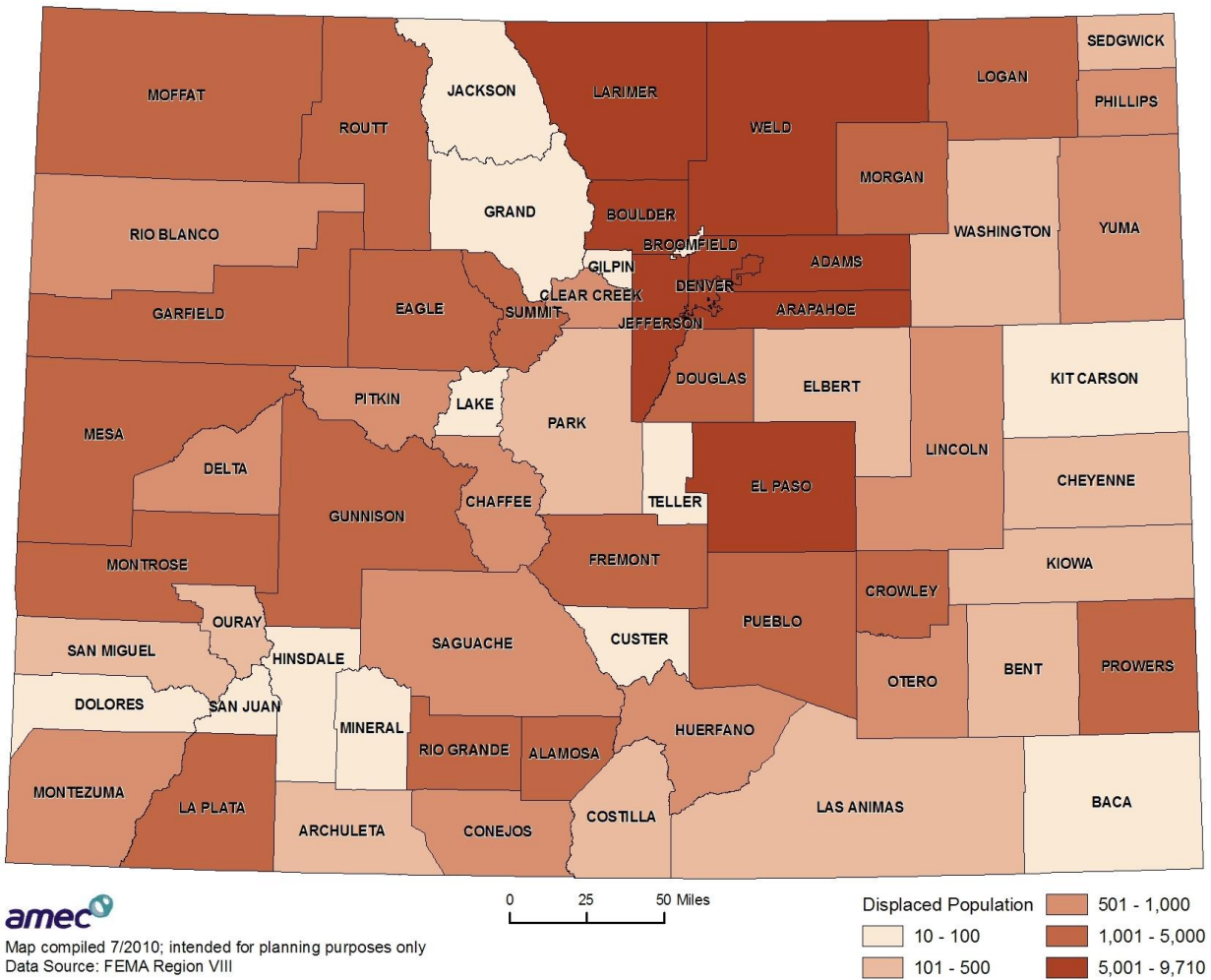
Figure 12 Displaced Population by County based on HAZUS
